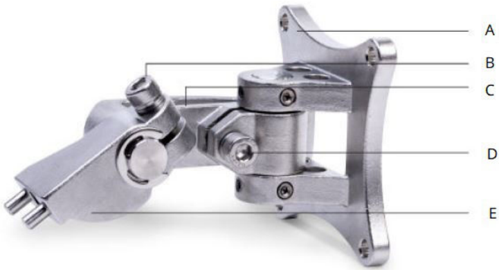
Figure 2-1: Tilt mount
