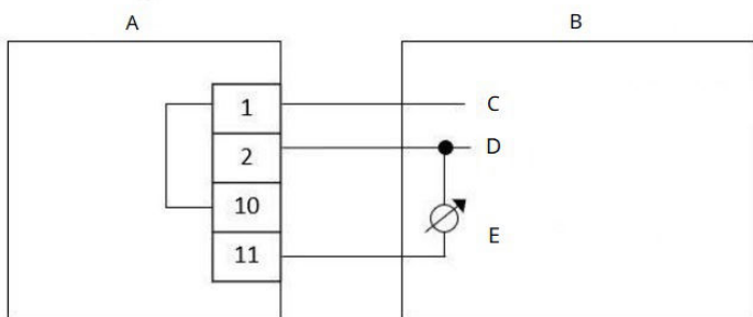
Figure 2-7: Source three-wire
