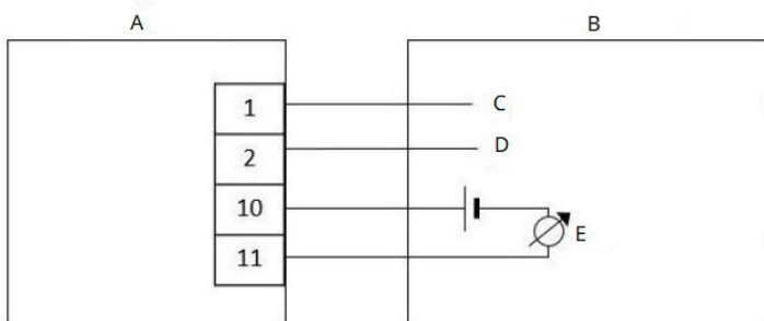
Figure 2-6: Sink four-wire
